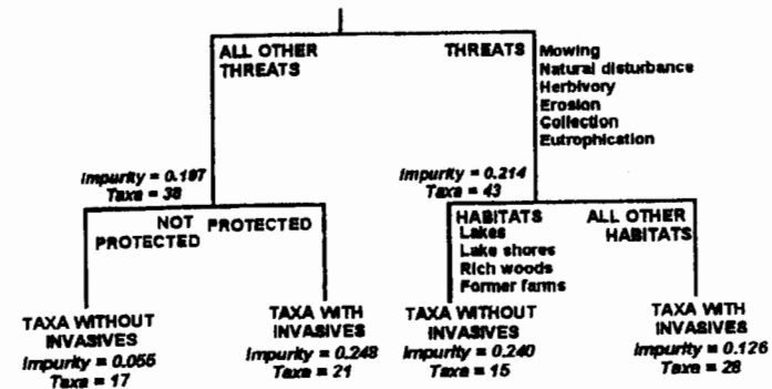
Figure 3. Classification tree showing the variable states that best distinguish species that exhibited co-occurring invasives and those that were free of invasives ( N = 81 species). Numbers of taxa at each node show the number of cases that were split into "uninvaded" and "invaded" categories by each splitting variable. The first bifurcation was on the presence of all threats (see text for details). Bifurcations then proceeded on protection status (held or not held by a conservation entity) and habitat type (listed in the figure). Misclassification rates (impurity levels) ranged from 0.055 to 0.248 at each node. Overall model PRE was 0.347.
